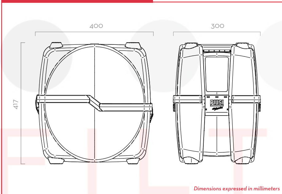
ROTATING CONNECTION
